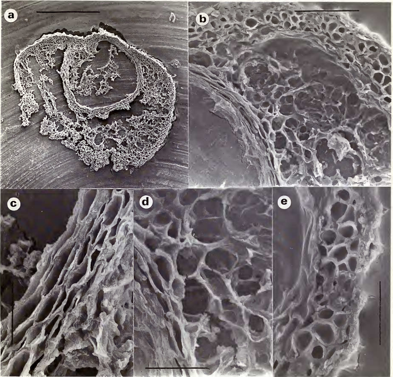
Fig. 56 Sarcopyrenia gibba (Nyl.) Nyl. (H-NYL 4058—lectotype) (a) Vertical section of ascoma; scale = 200 \mu\text{m} ; (b) Detail of exciple: 3-layered wall, textura angularis; scale = 43 \mu\text{m} ; (c) Detail of inner layer: textura angularis with laterally compressed cells; scale = 17.6 \mu\text{m} ; (d) Detail of middle layer: textura angularis; scale = 20 \mu\text{m} ; (e) Detail of outer layer: textura angularis; scale = 20 \mu\text{m} .
